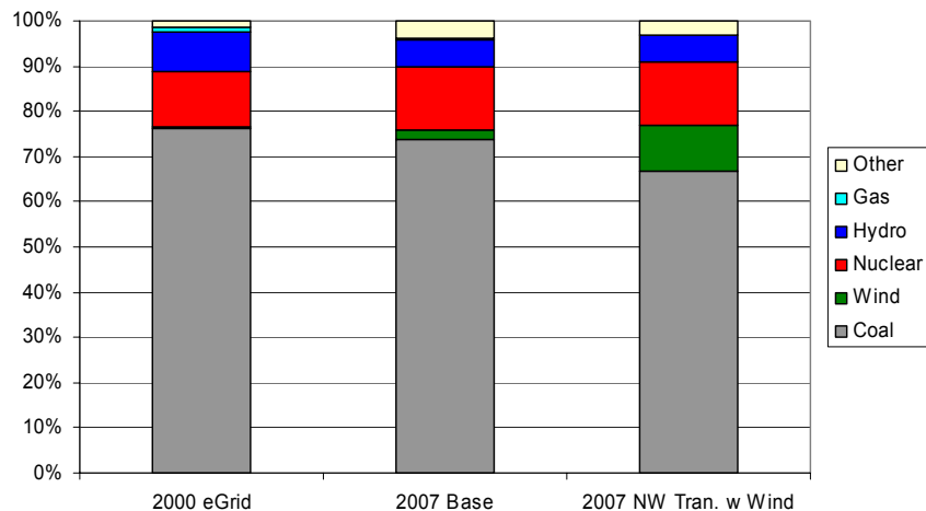
Generation Fuel Mix (% GWh)
