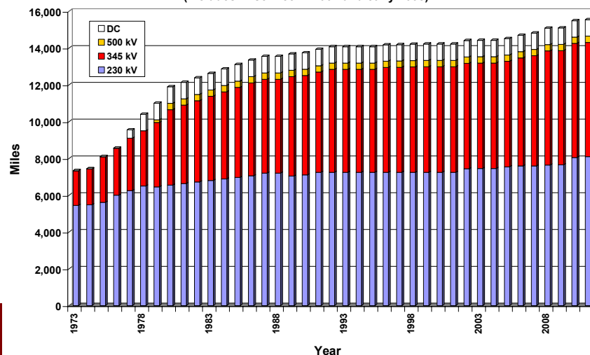
MAPP-US Miles of Line Over 200 kV History Through 2001 and Expected Additions From MAPP 2003 Update Report (includes In-service in 2002 and early 2003)
